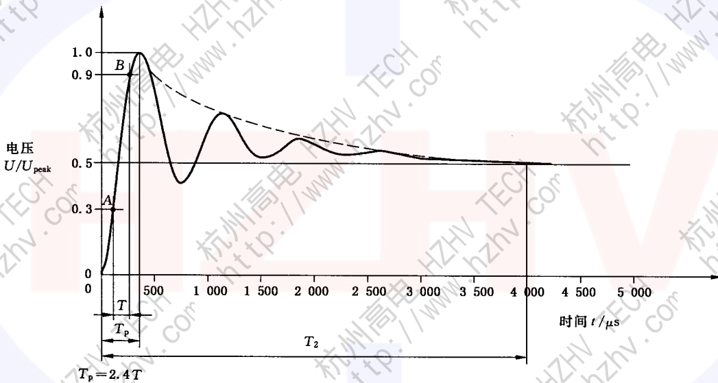
b) T_p/T_2 = 400/4\ 000\ \mu\text{s}, 1\ \text{kHz}
