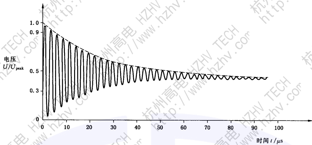
a) T_1/T_2 = 0.8/40 \mu\text{s}, 370 \text{ kHz}
